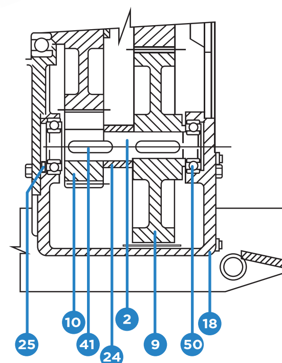
LAY SHAFT ASSEMBLY
